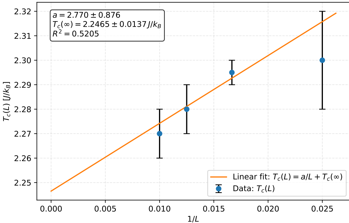
Finite-size scaling of T_c(L) vs 1/L
