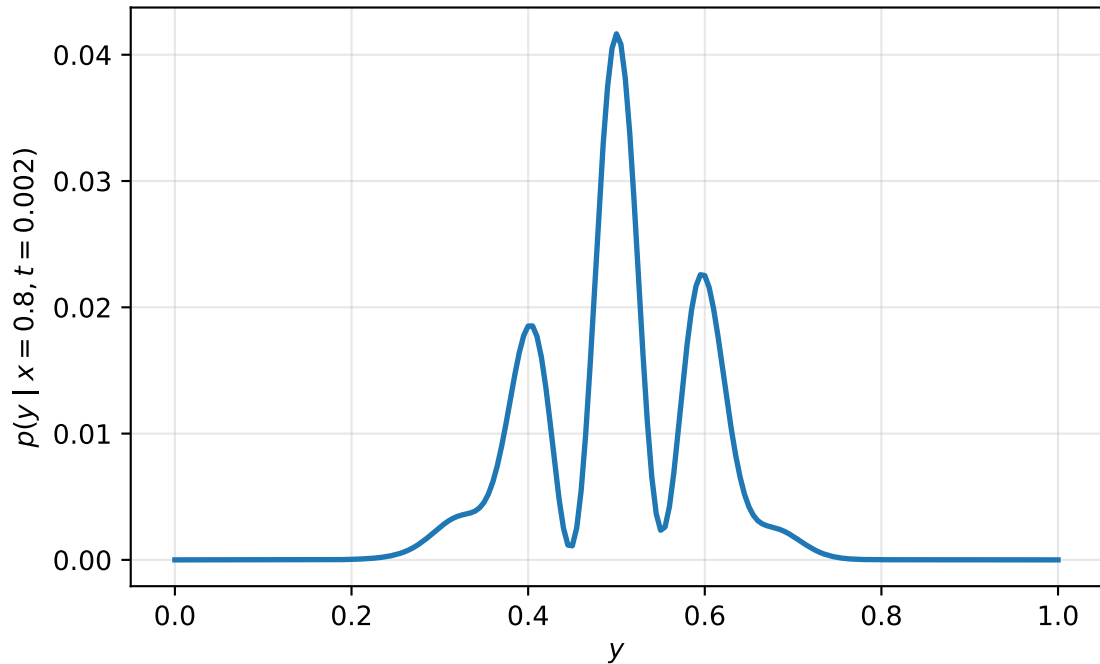
Double-slit detection probability along screen at x = 0.8
