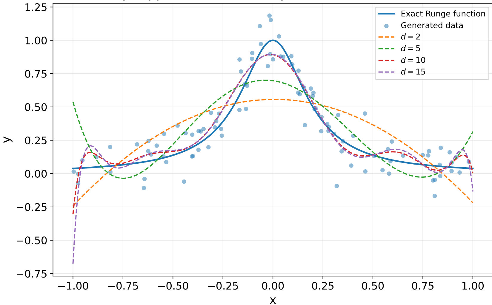
Ridge approximation of Runge's function ( \lambda = 1e - 06 )
