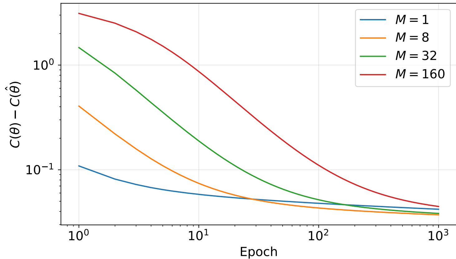
OLS SGD: inverse time schedule
