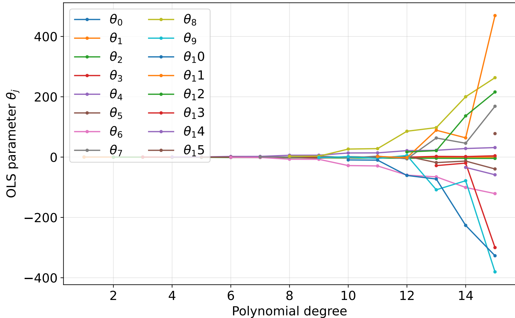
OLS parameters vs polynomial degree ( n = 100 , \sigma = 0.1 )
