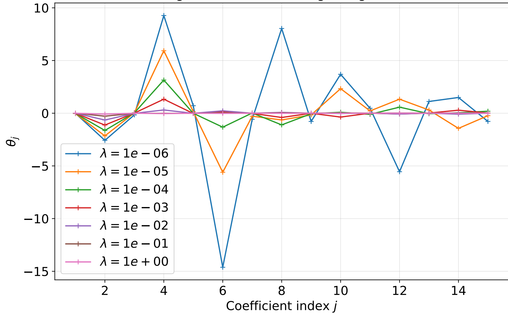
Ridge coefficient shrinkage, degree 15
