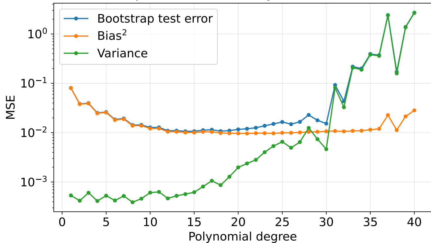
Bootstrap bias--variance analysis ( n = 400 , \sigma = 0.1 )
