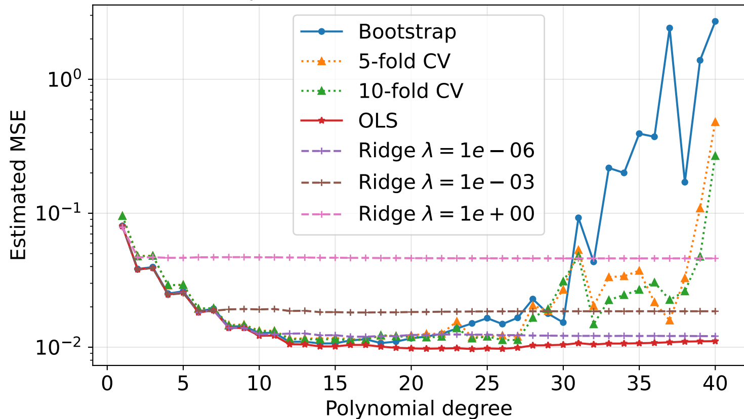
Bootstrap and cross-validation ( n = 400 , \sigma = 0.1 )
