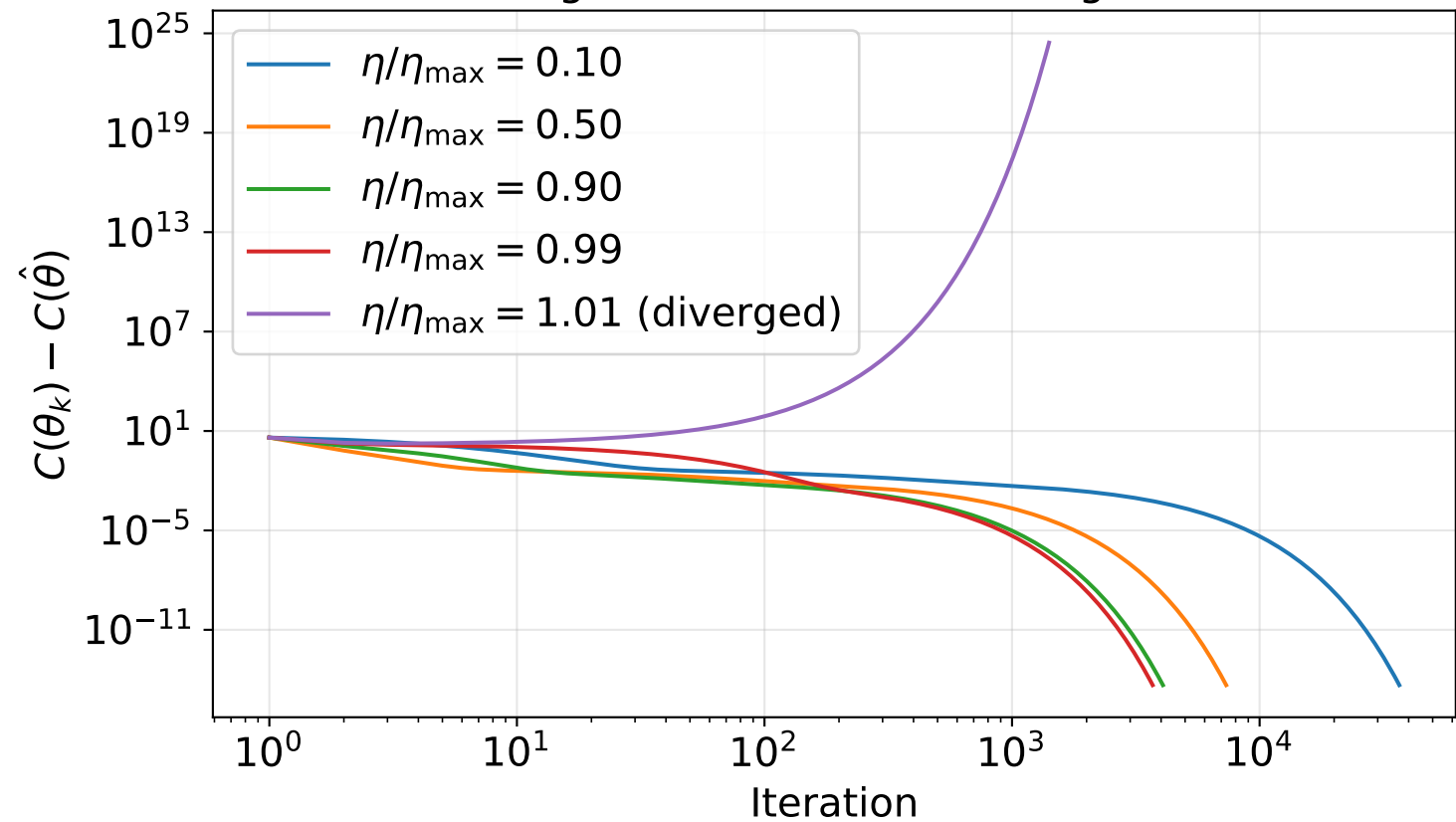
OLS gradient-descent convergence
