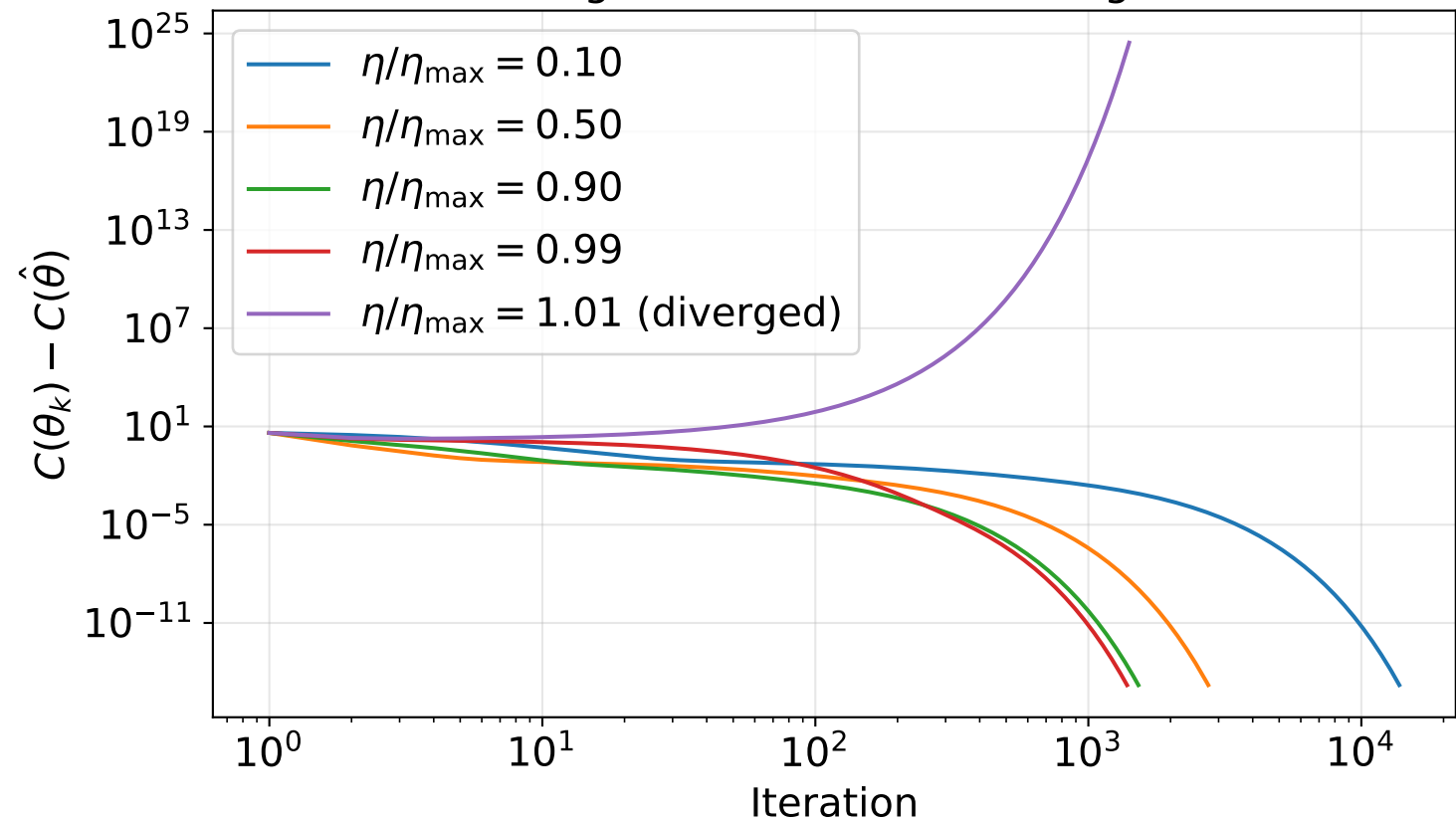
RIDGE gradient-descent convergence
