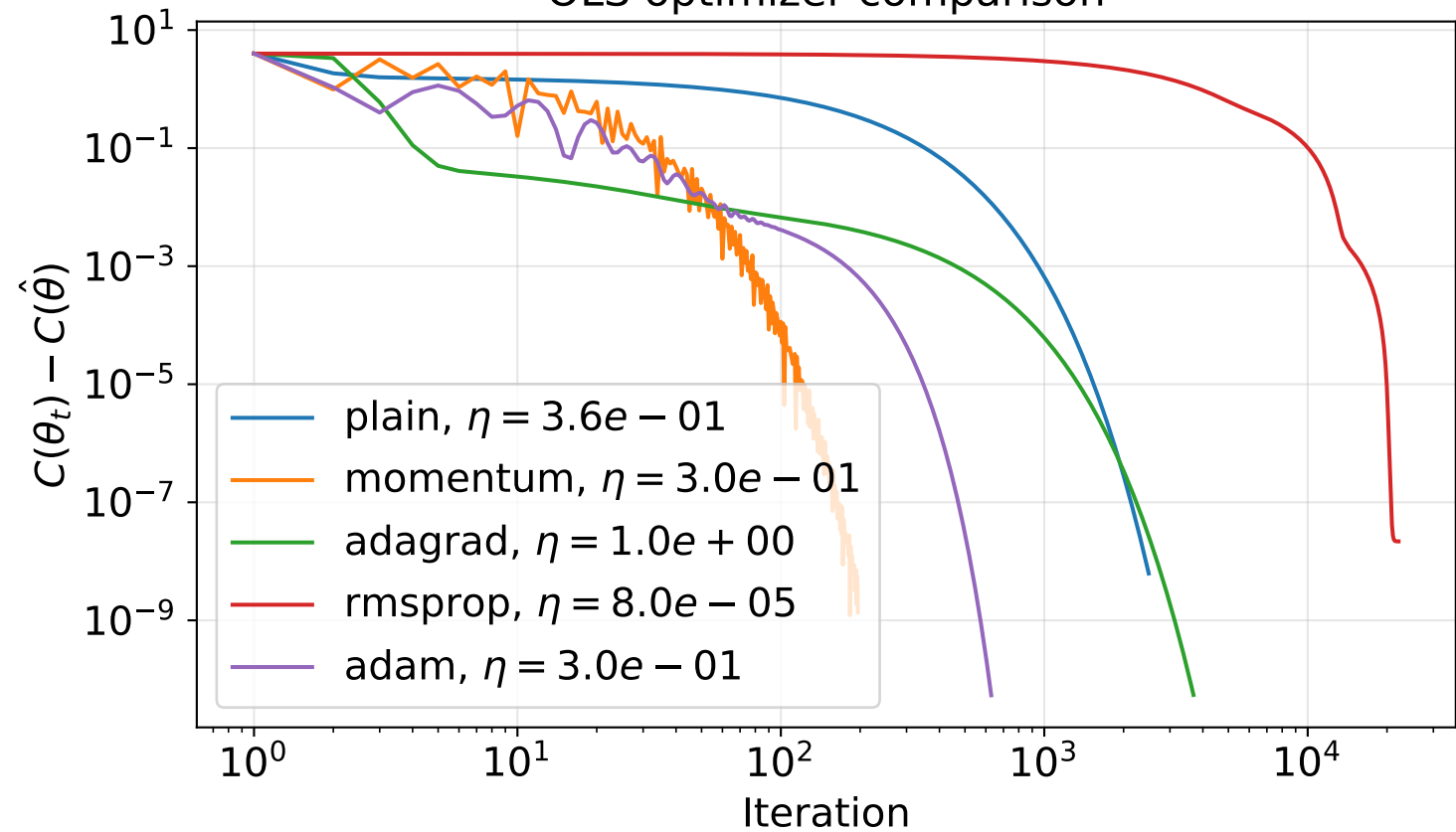
OLS optimizer comparison
