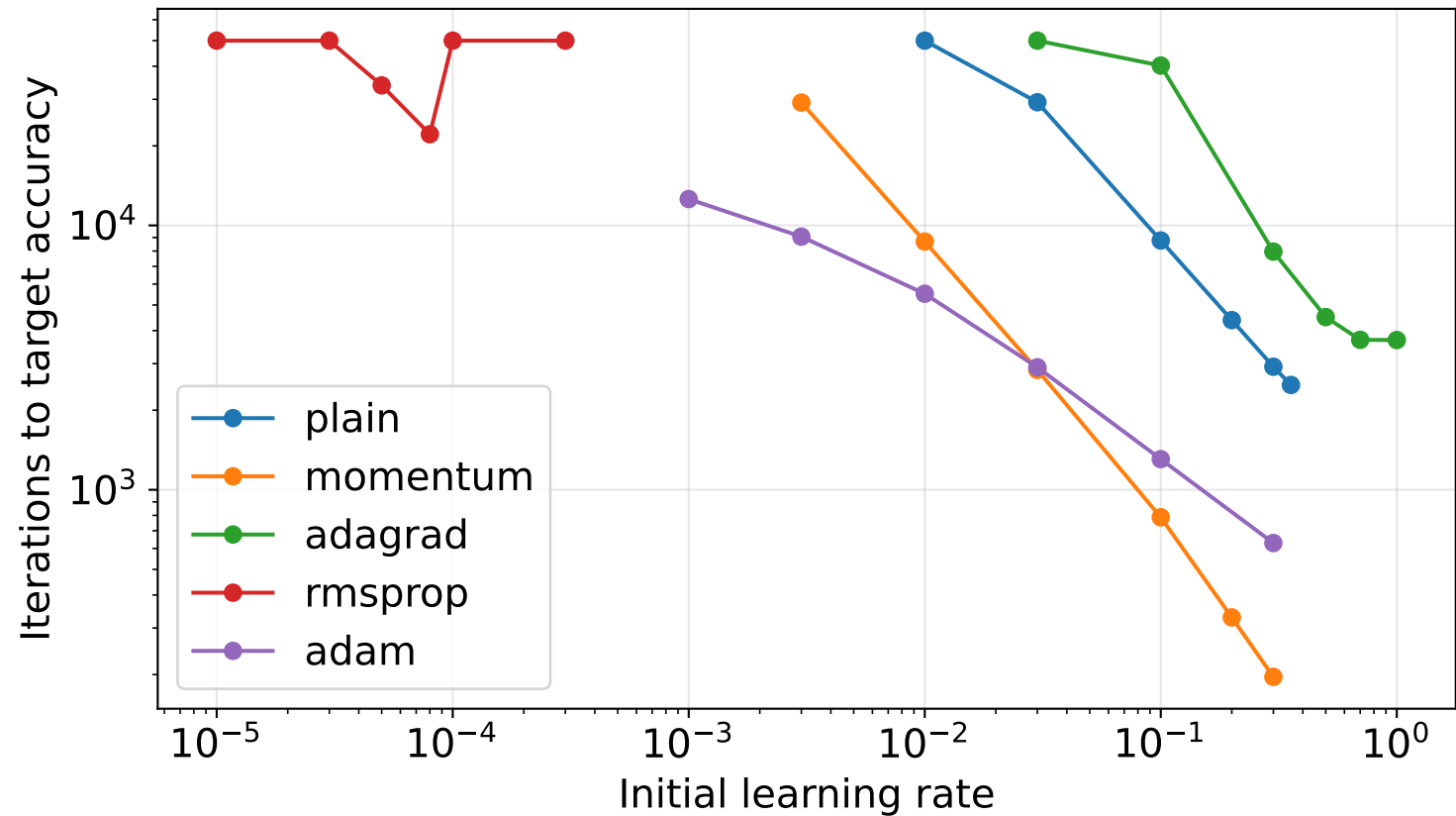
OLS learning-rate sensitivity ( \varepsilon_{\theta} = 1e - 04 )
