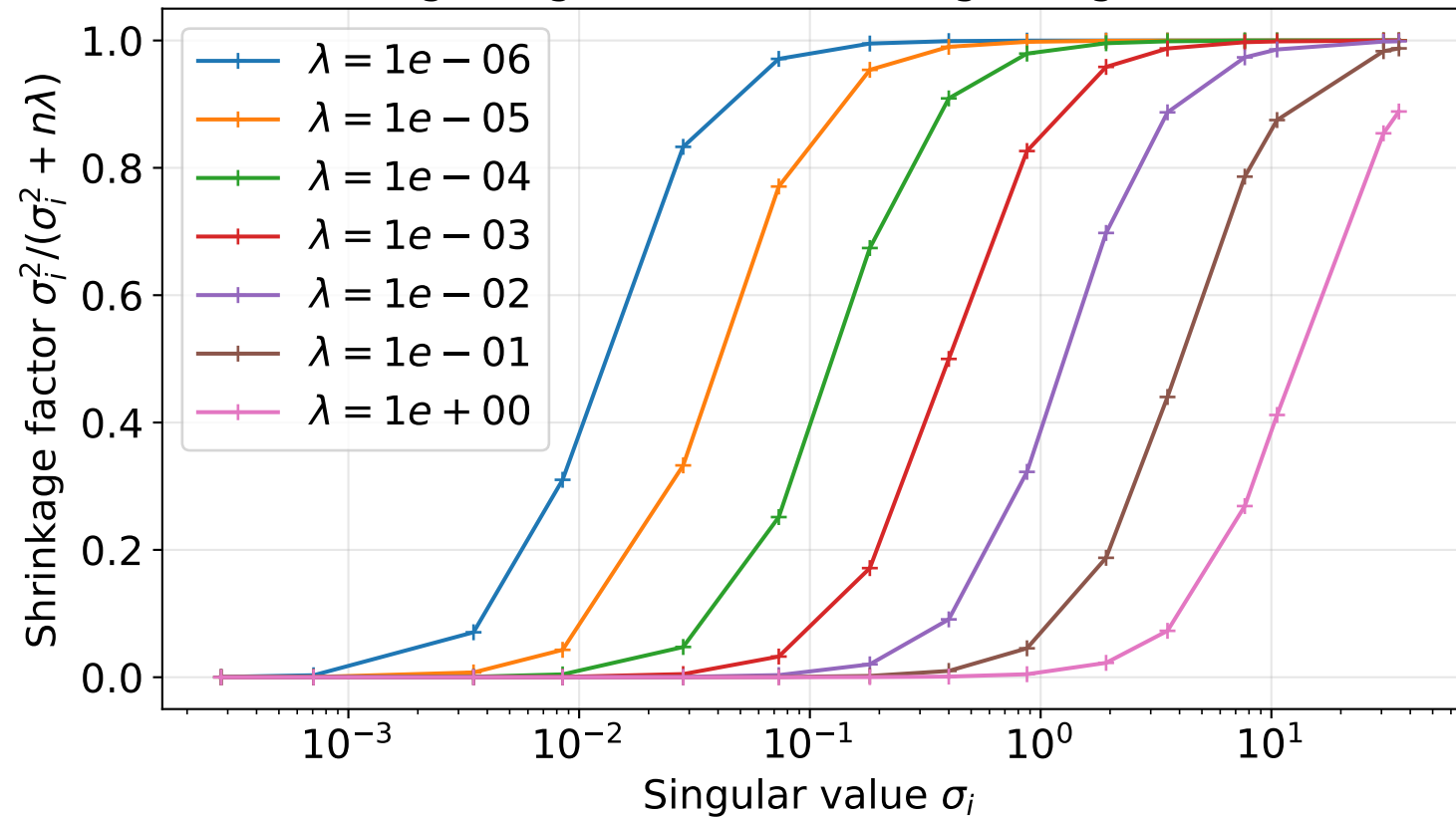
Ridge singular-value shrinkage (degree 15)
