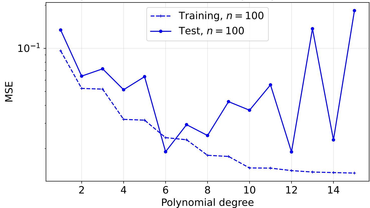
Training and test error vs model complexity ( n = 100 , \sigma = 0.1 )
