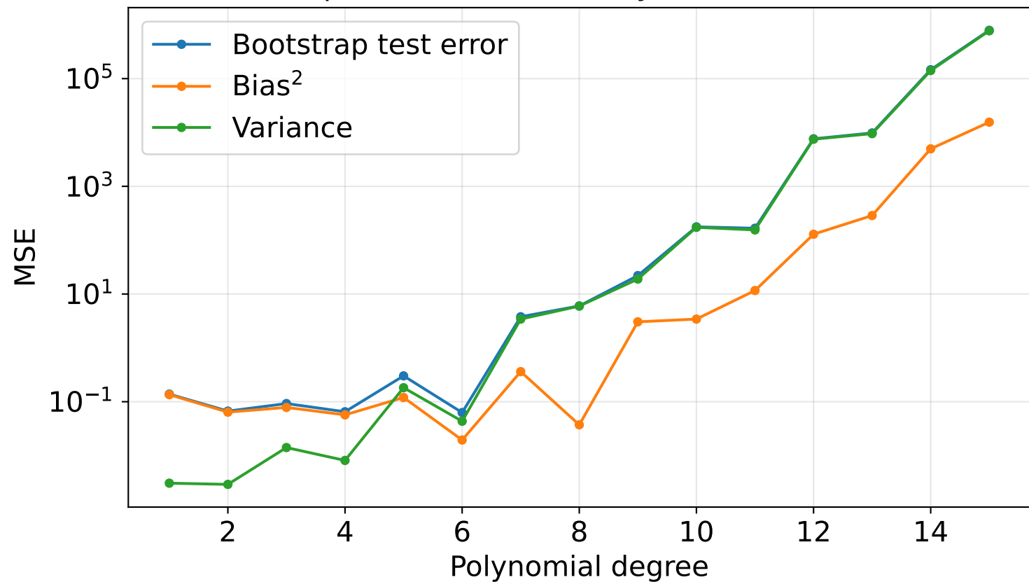
Bootstrap bias--variance analysis ( n = 100 , \sigma = 0.1 )
