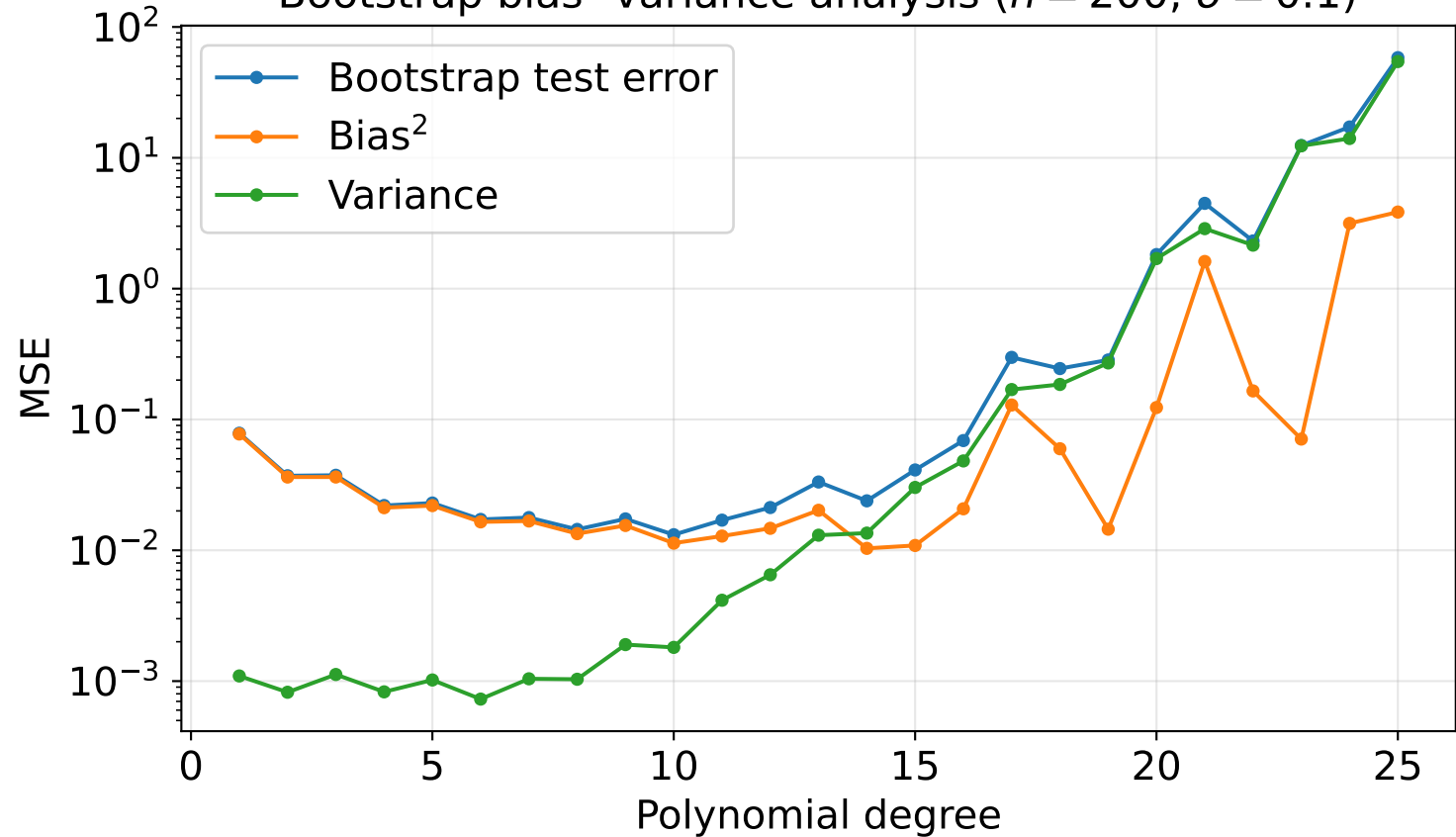
Bootstrap bias--variance analysis ( n = 200 , \sigma = 0.1 )
