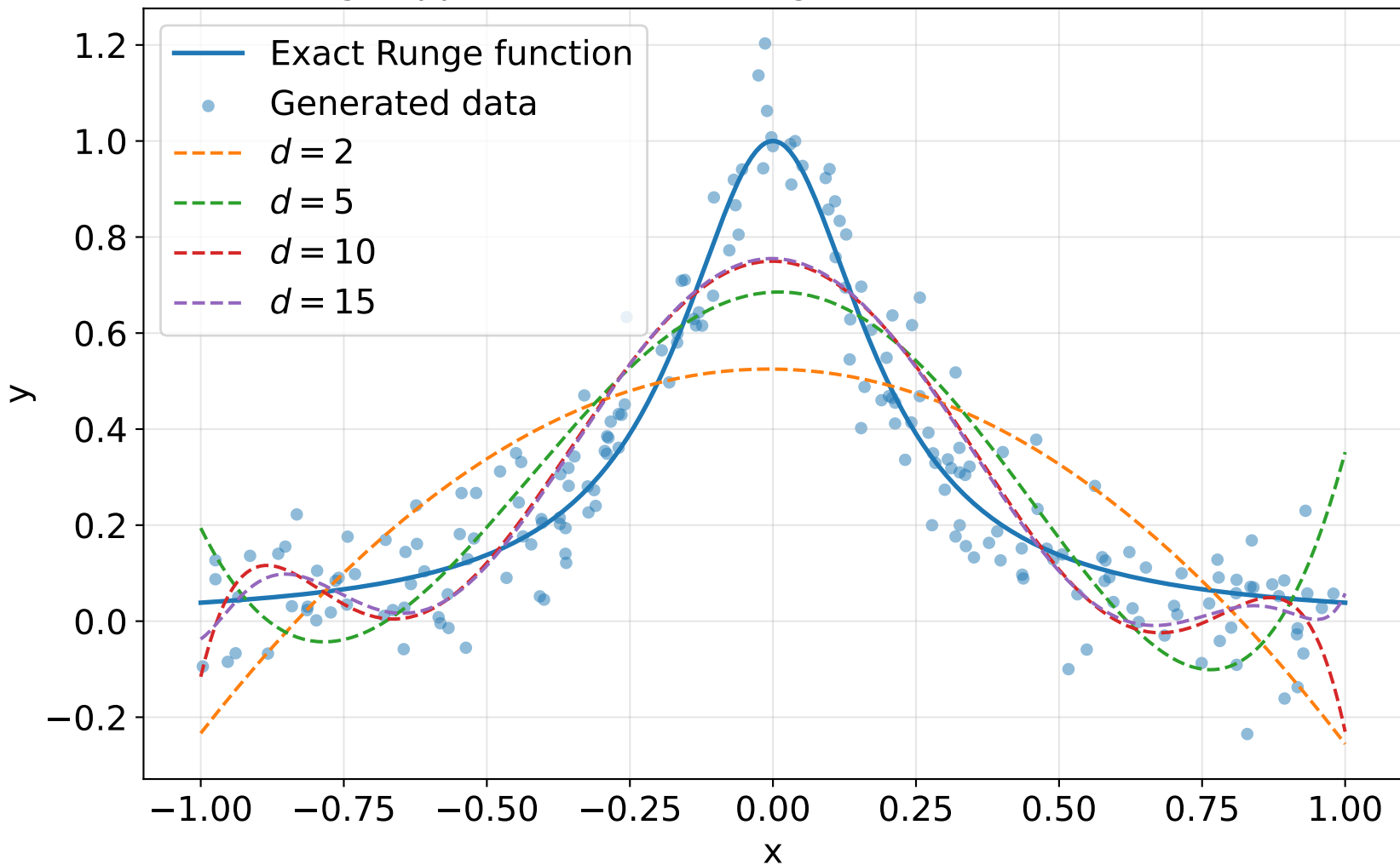
Ridge approximation of Runge's function ( \lambda = 1e - 03 )
