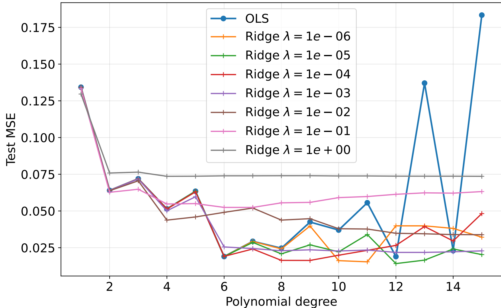
OLS and Ridge regression ( n = 100 , \sigma = 0.1 )
