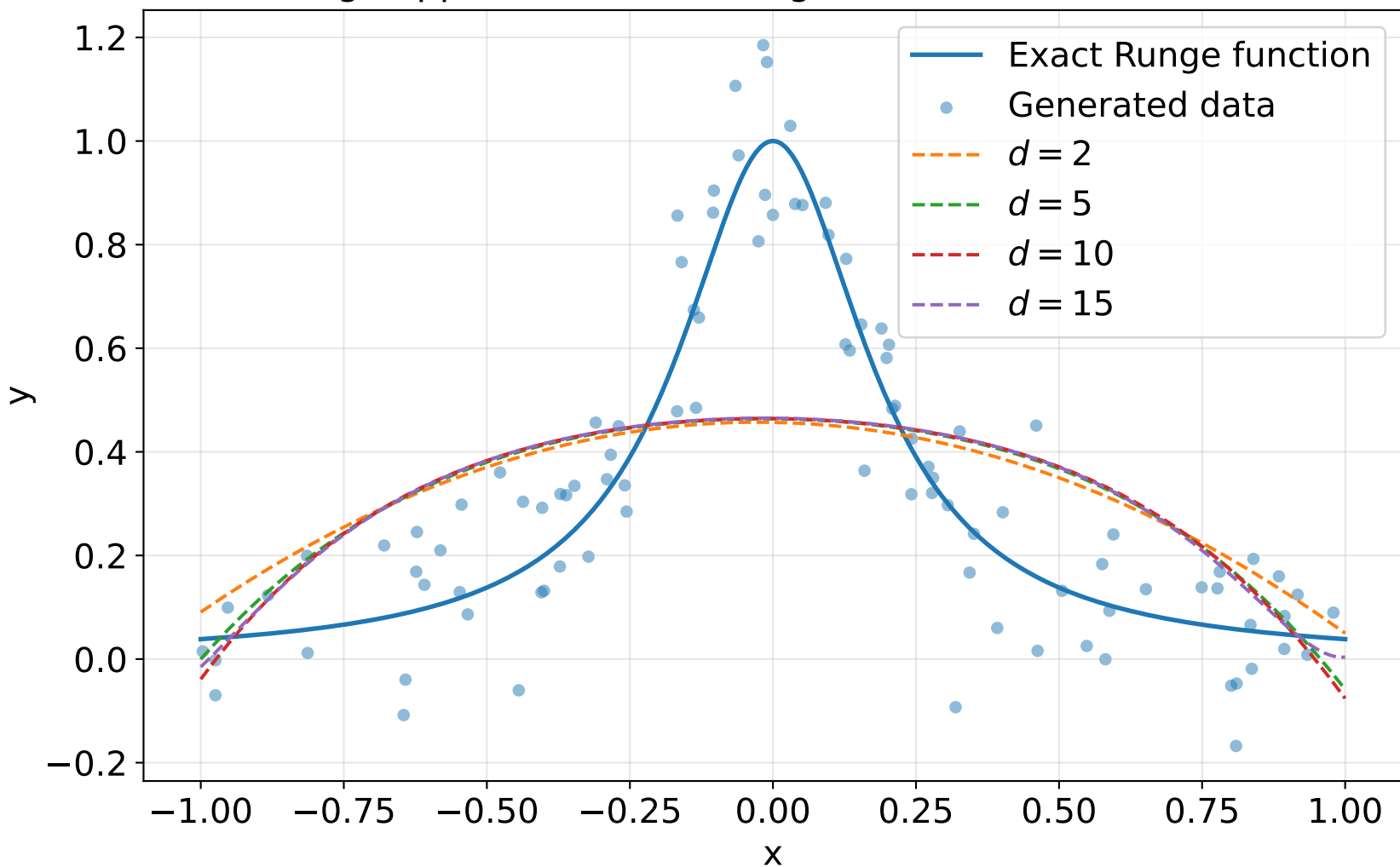
Ridge approximation of Runge's function ( \lambda = 1e + 00 )
