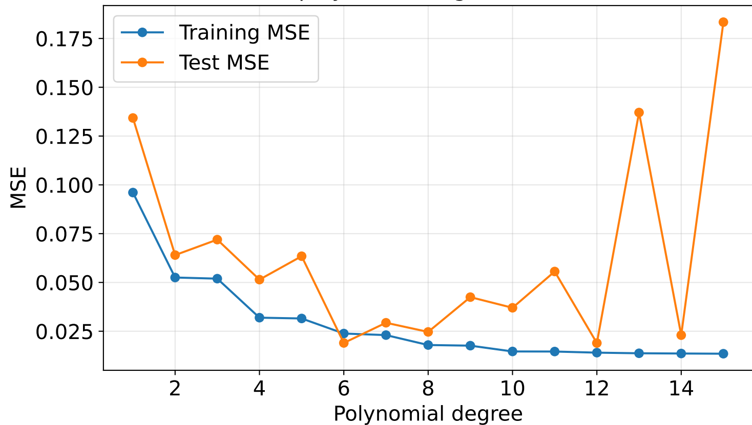
OLS: MSE vs polynomial degree ( n = 100 , \sigma = 0.1 )
