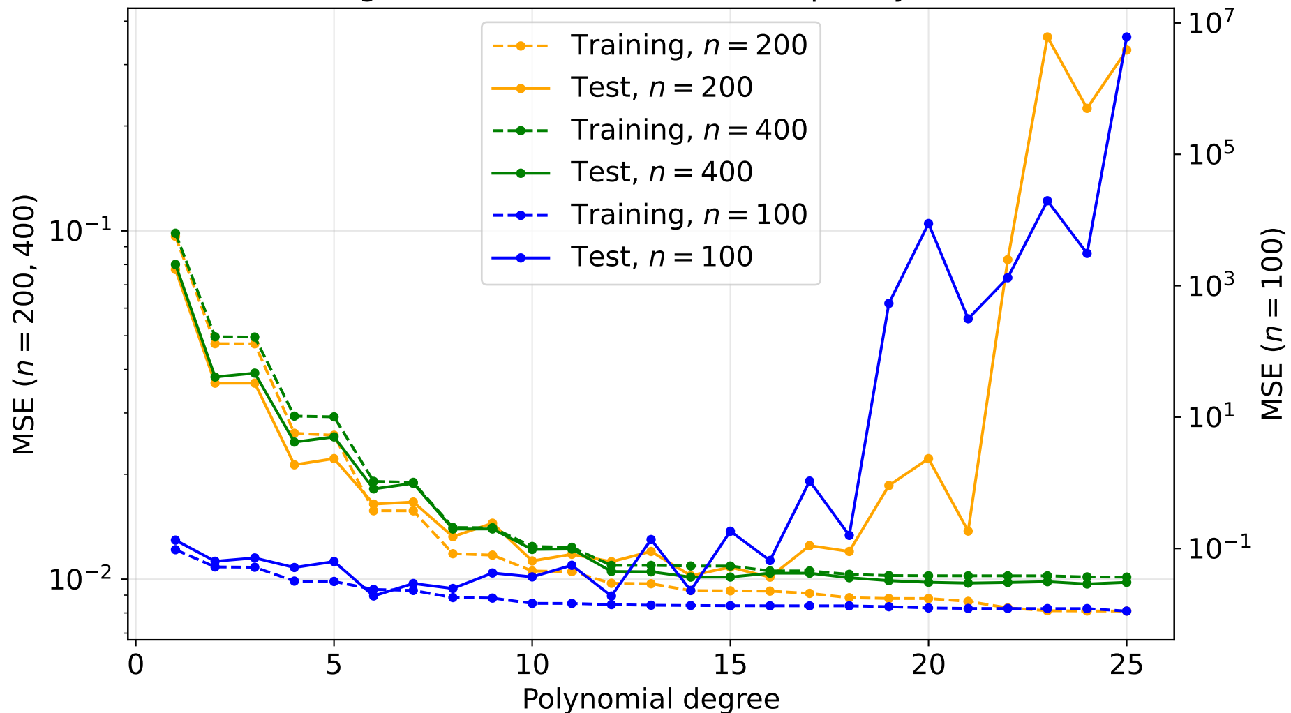
Training and test error vs model complexity ( \sigma = 0.1 )
