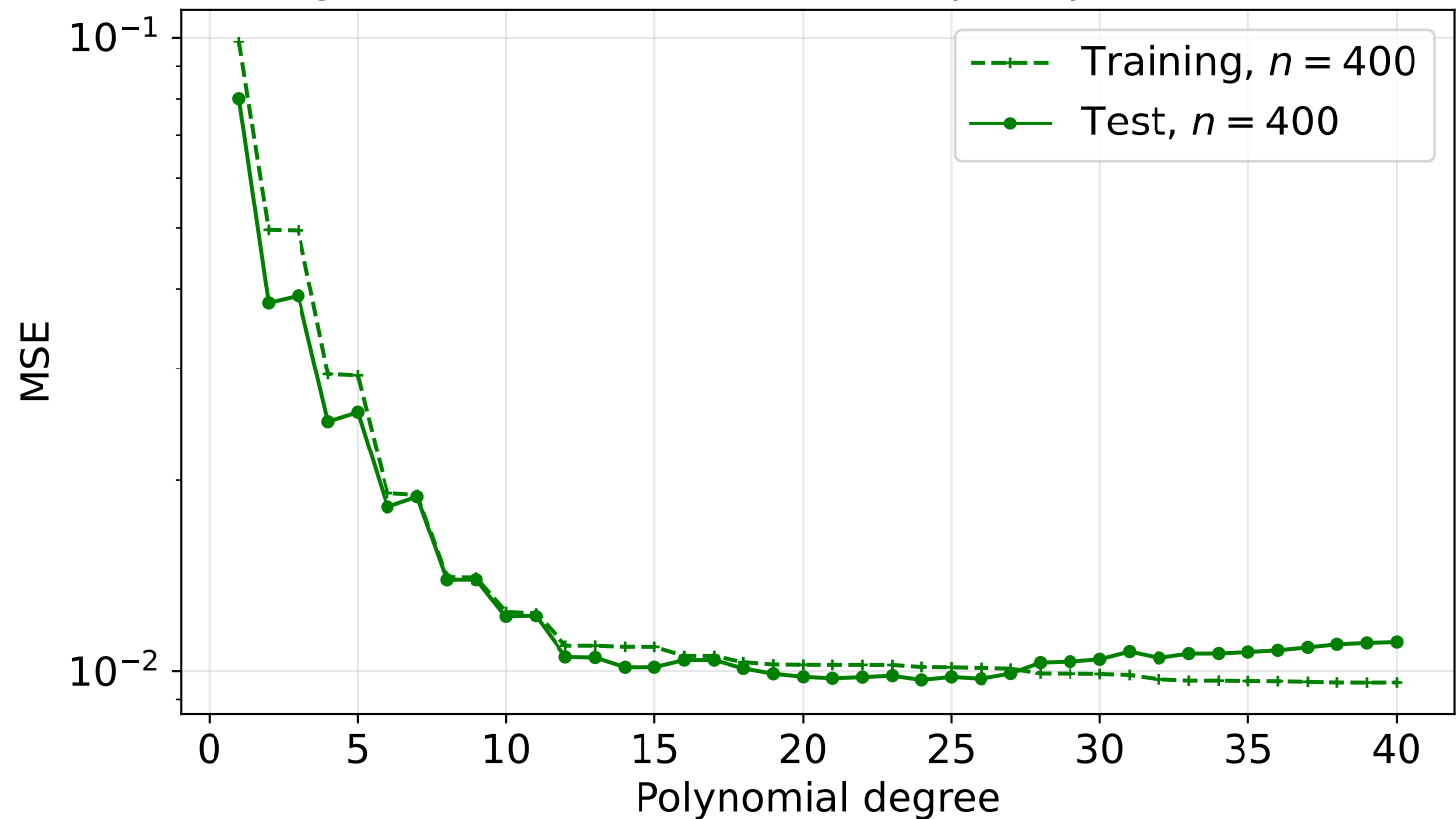
Training and test error vs model complexity ( n = 400 , \sigma = 0.1 )
