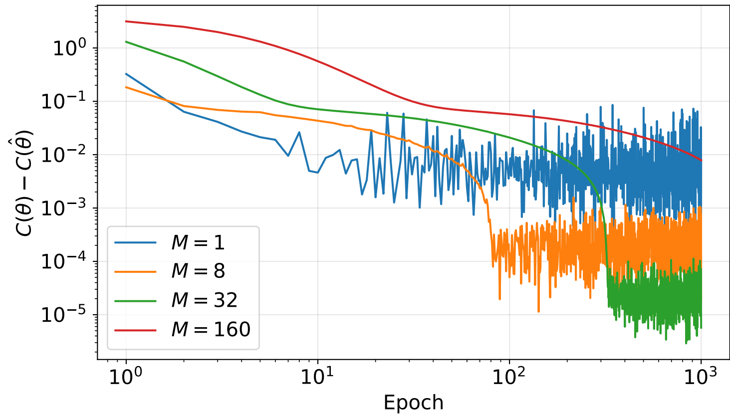
LASSO SGD: constant schedule
