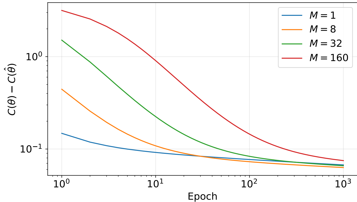
RIDGE SGD: inverse time schedule
