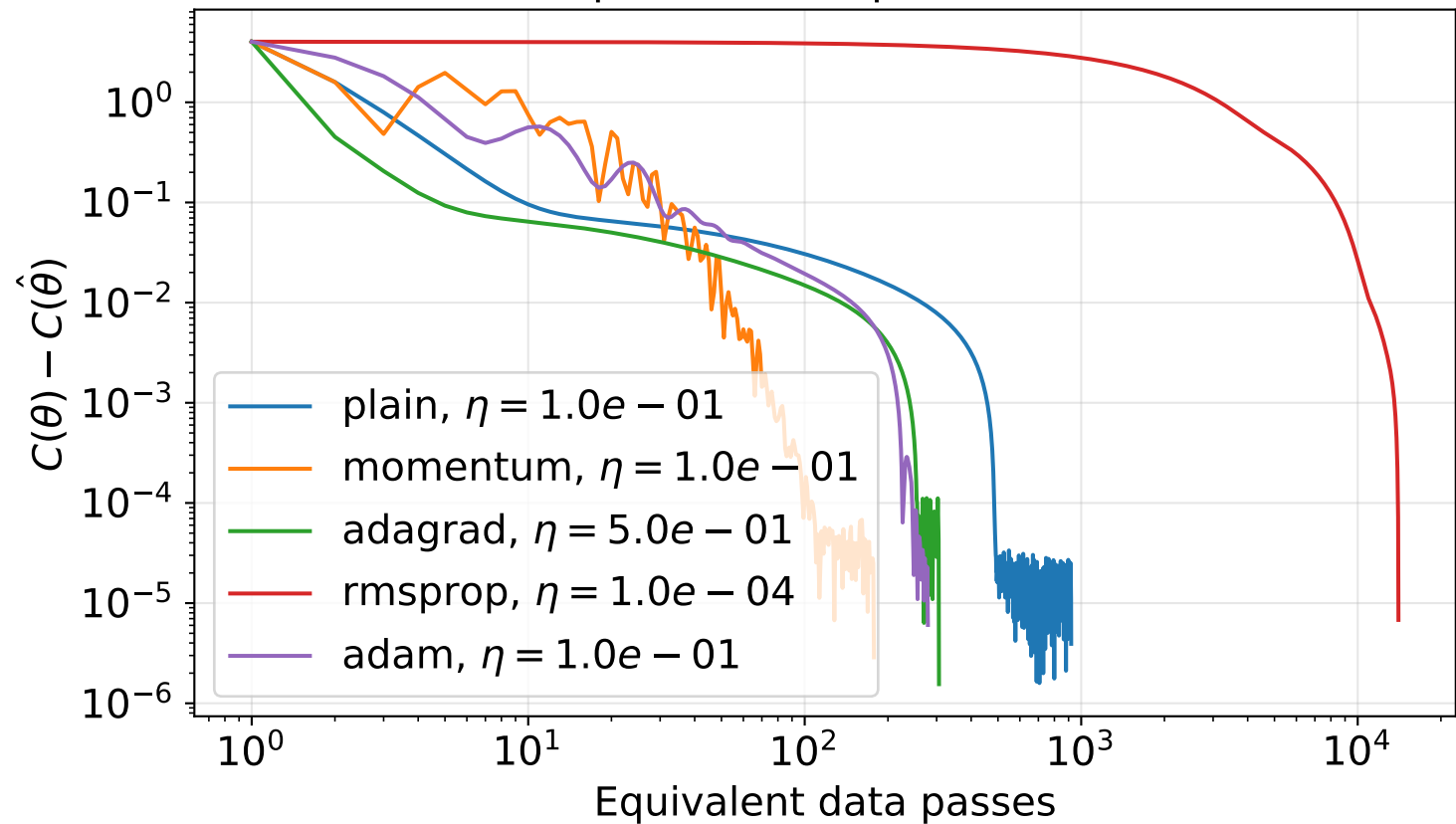
LASSO optimizer comparison with SGD
