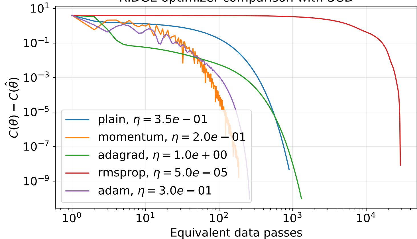
RIDGE optimizer comparison with SGD
