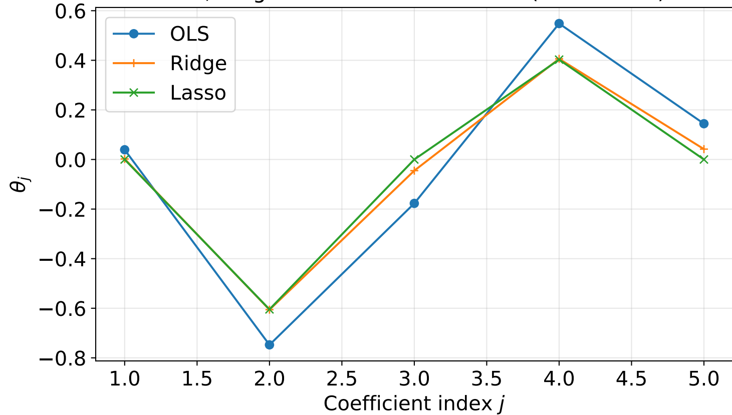
OLS, Ridge and Lasso coefficients ( \lambda = 1e - 02 )
