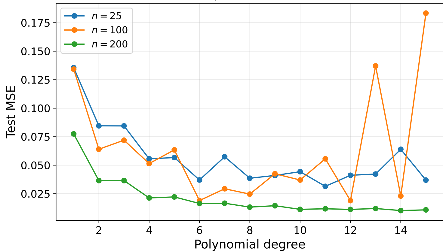
Effect of sample size on OLS ( \sigma = 0.1 )
