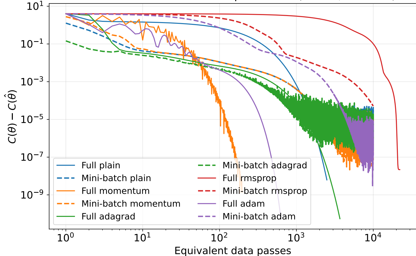
OLS: full-batch vs mini-batch optimization ( M = 32 , constant)
