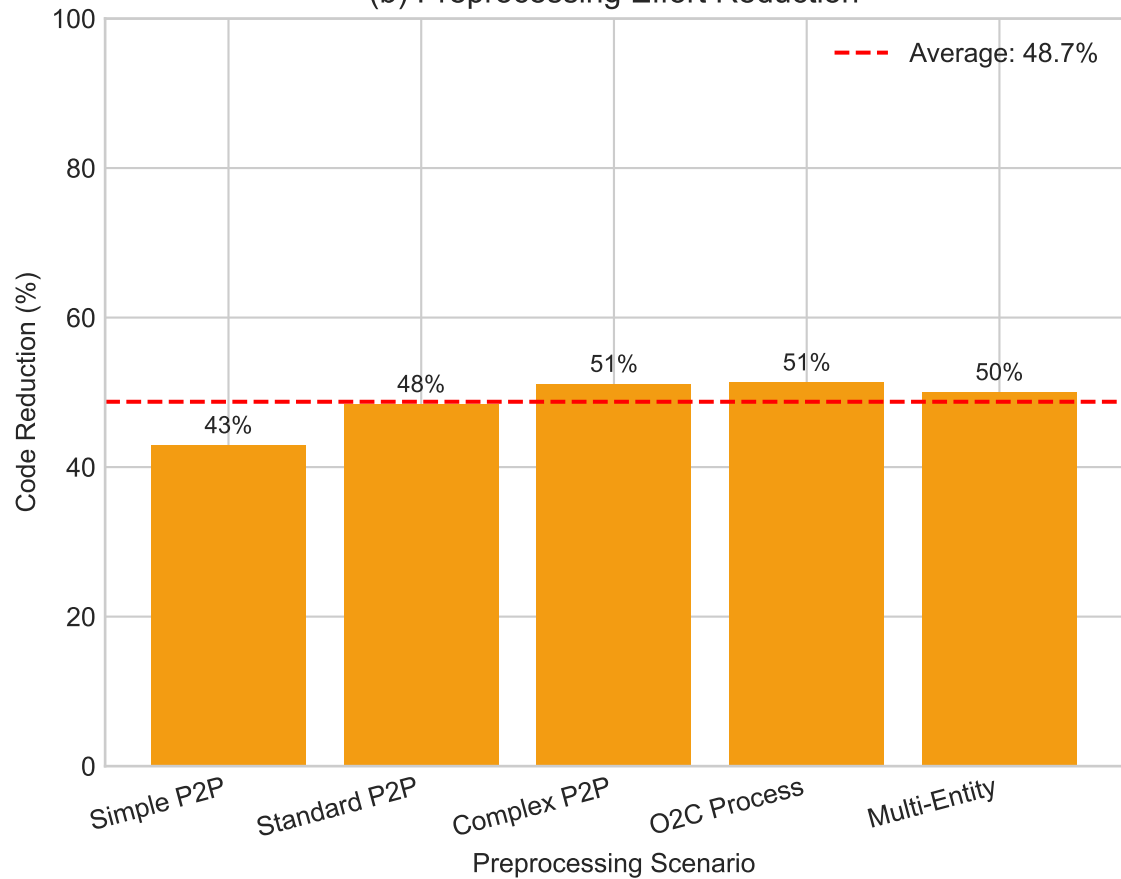
(b) Preprocessing Effort Reduction
