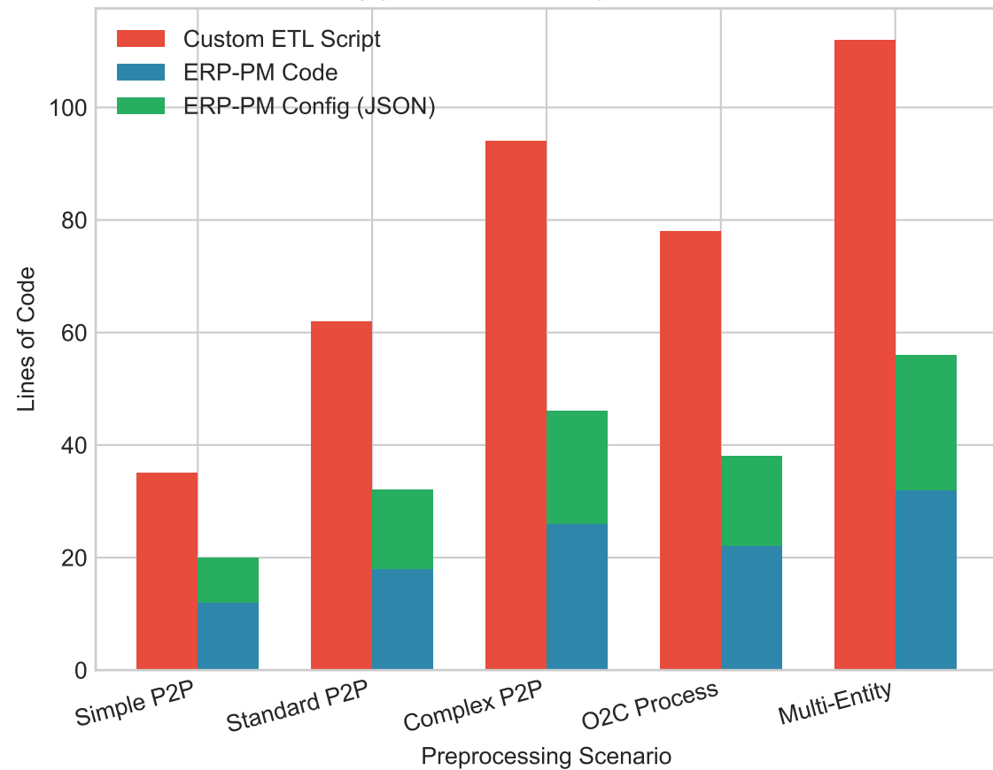
(a) Lines of Code by Approach
