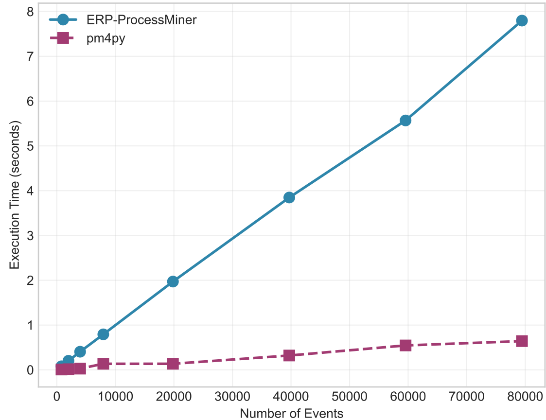
(a) Total Execution Time vs. Log Size
