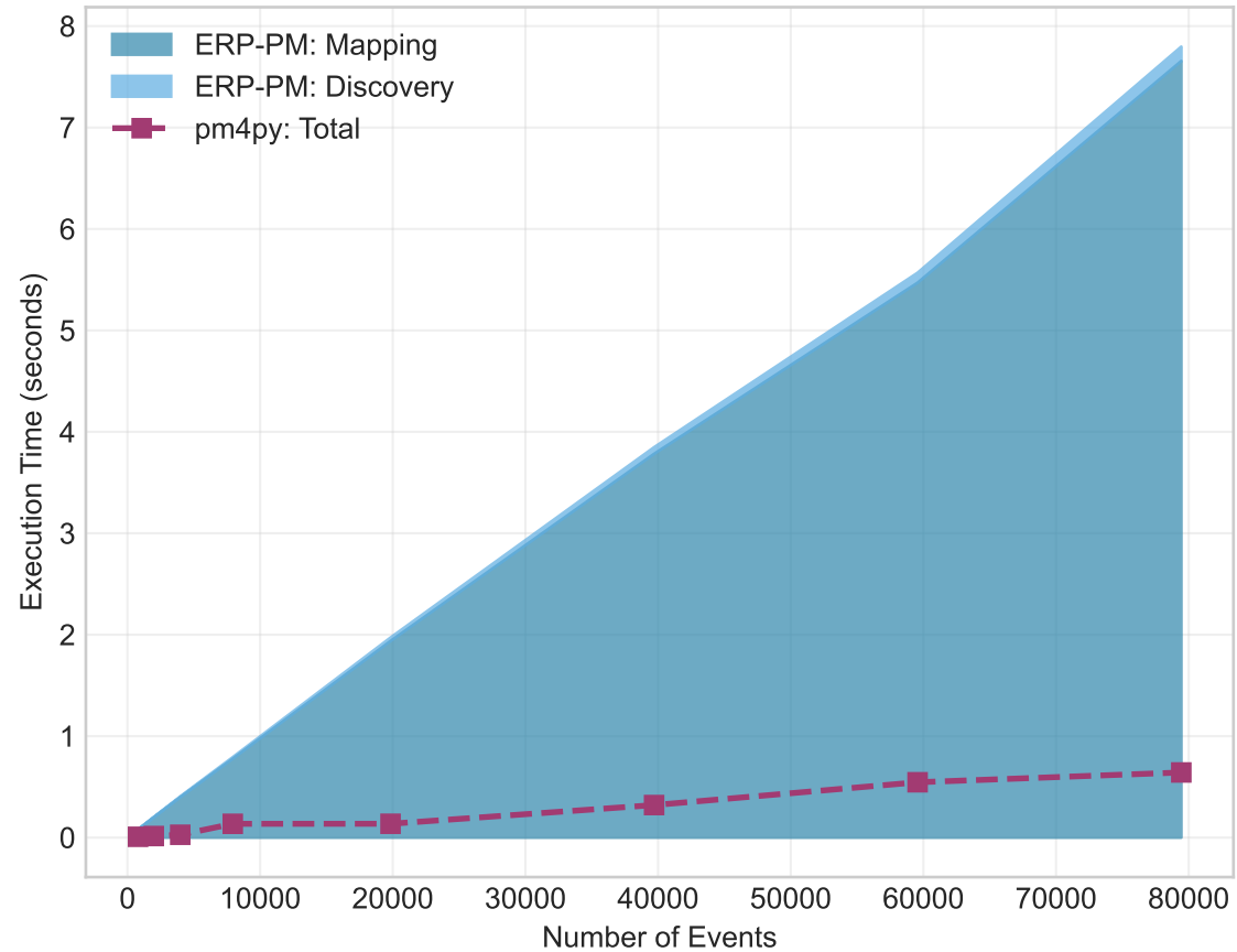
(b) Time Breakdown Analysis
