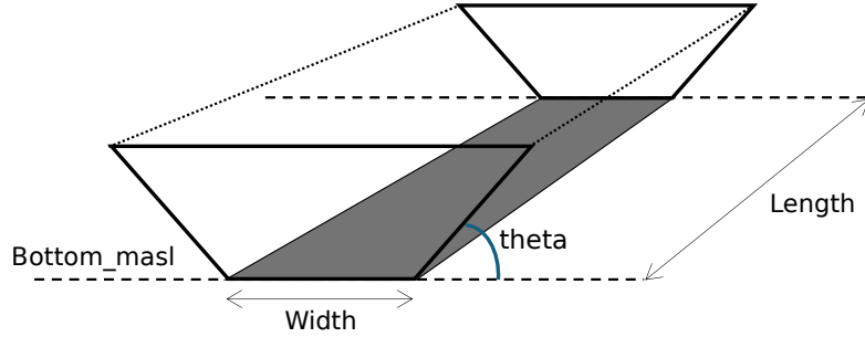
Figure 2.3: Reservoir with parametric geometry
