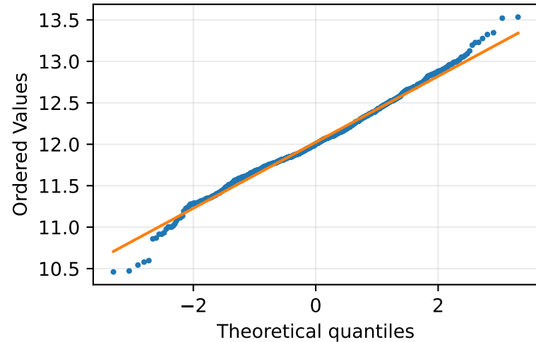
Q-Q plot
