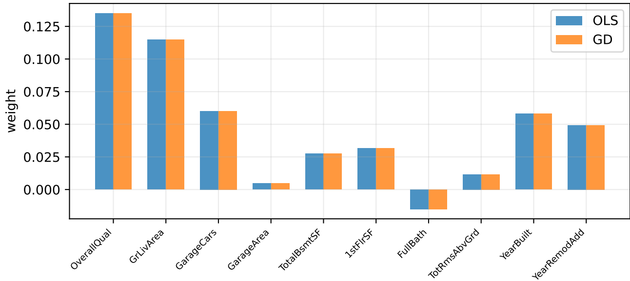
OLS vs GD weights
