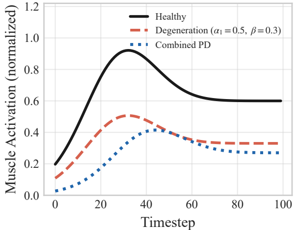
Muscle Activation
