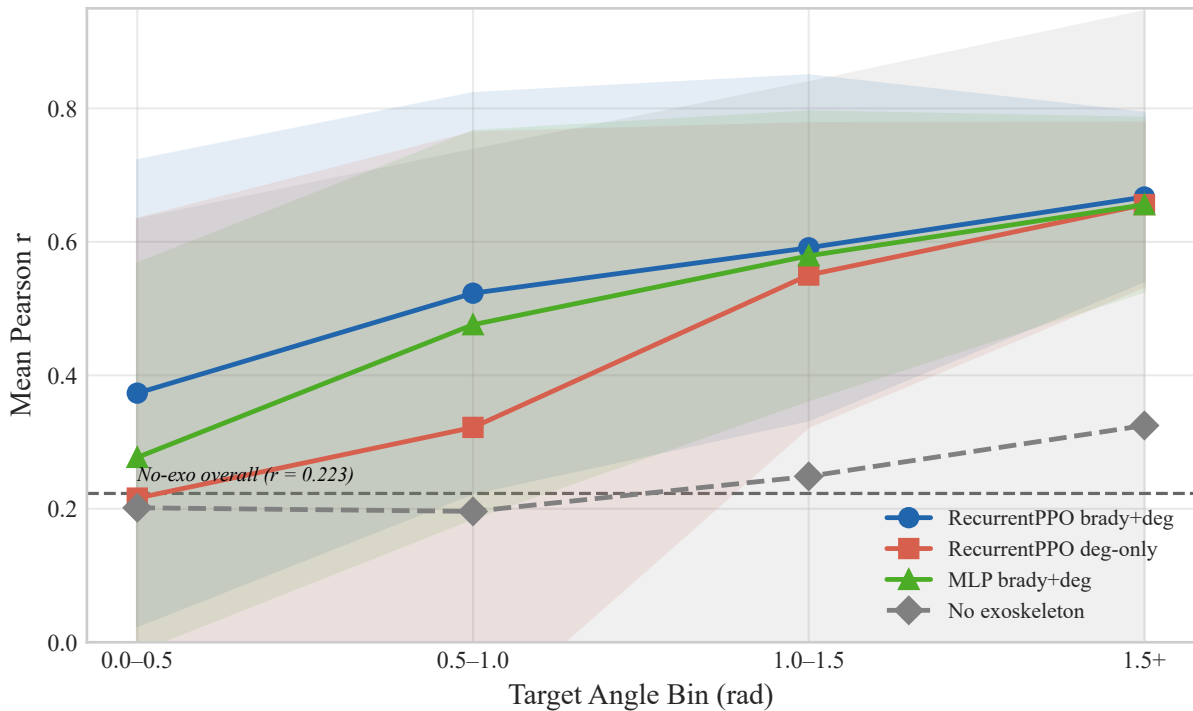
Trajectory Tracking vs. Target Angle
