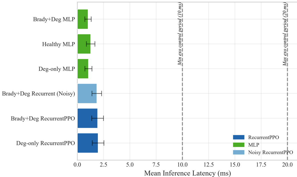
Per-Step Inference Latency vs. Real-Time Budget
