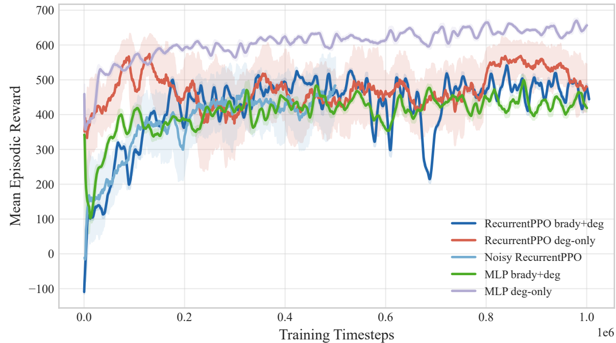
Training Reward Curves
