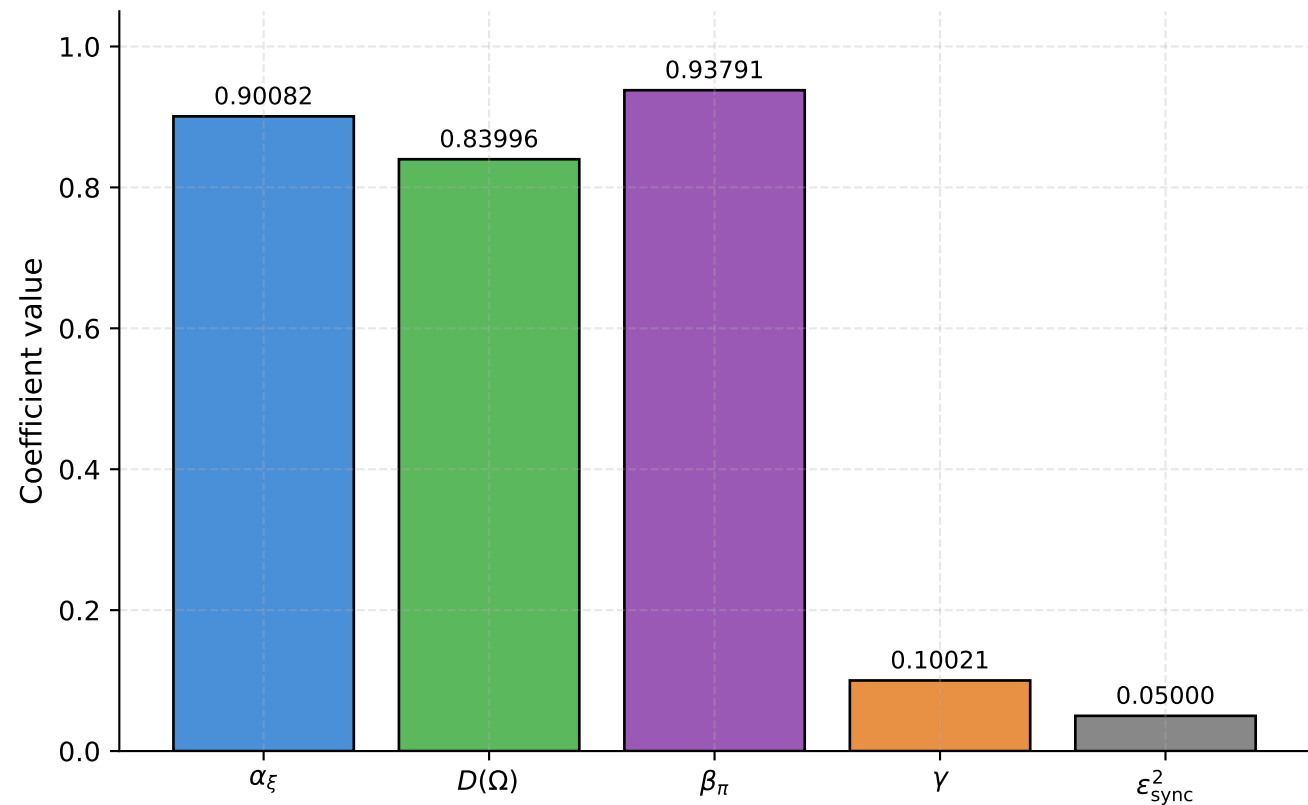
Five measured causal-wave transport coefficients
