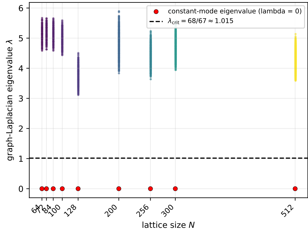
Lattice spectrum vs critical eigenvalue
