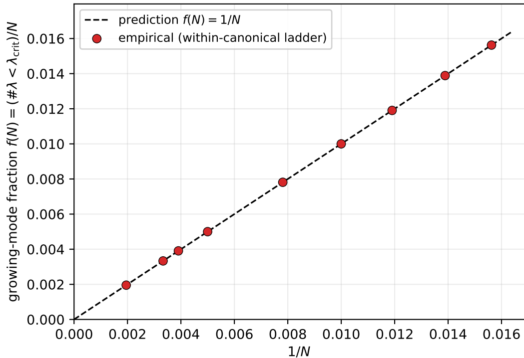
Symanzik convergence: f(N) = 1/N exactly
