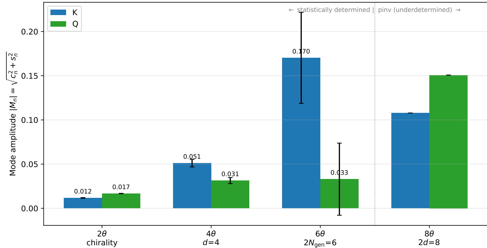
Fourier-mode spectrum of \langle K \rangle , \langle Q \rangle in chirality angle \theta_{\text{chir}}
