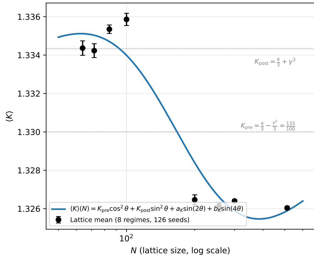
Factor field K : harmonic-basis System- \mathcal{R} closure
