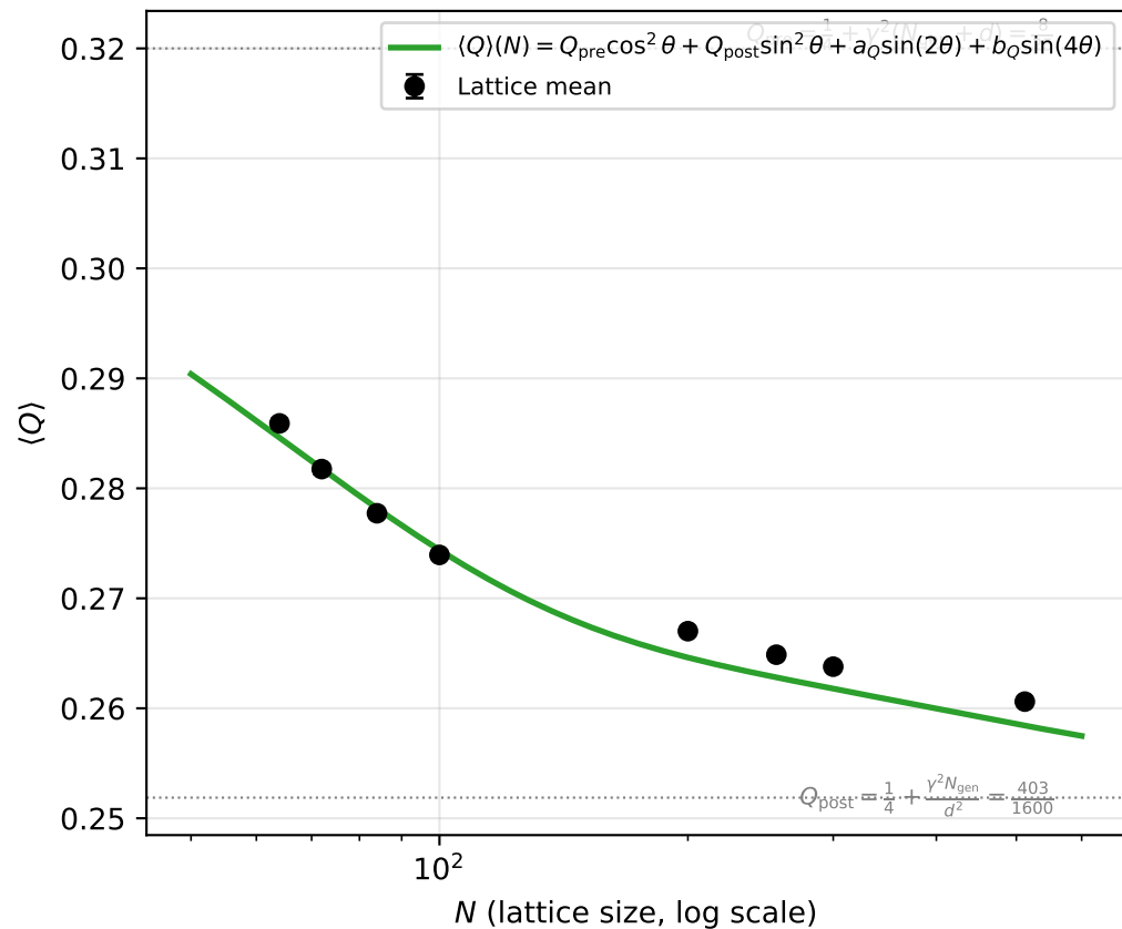
Factor field Q : harmonic-basis System- \mathcal{R} closure
