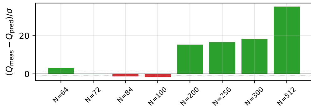
Residuals (constrained closure, 0 free parameters)
