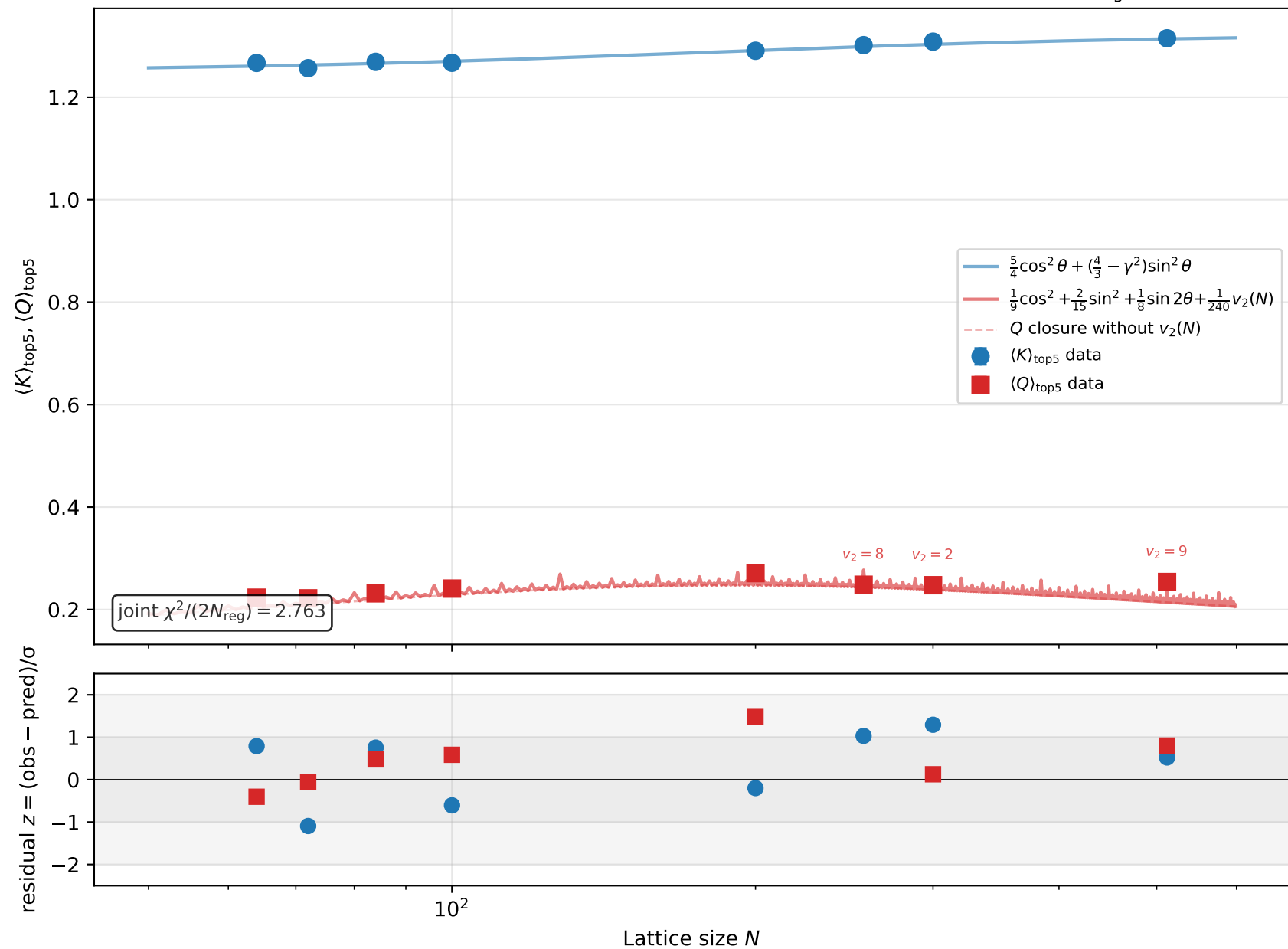
Matter-localised top-5\% closure of \langle K \rangle, \langle Q \rangle — zero free parameters in (\gamma, N_{\text{gen}}, d)
