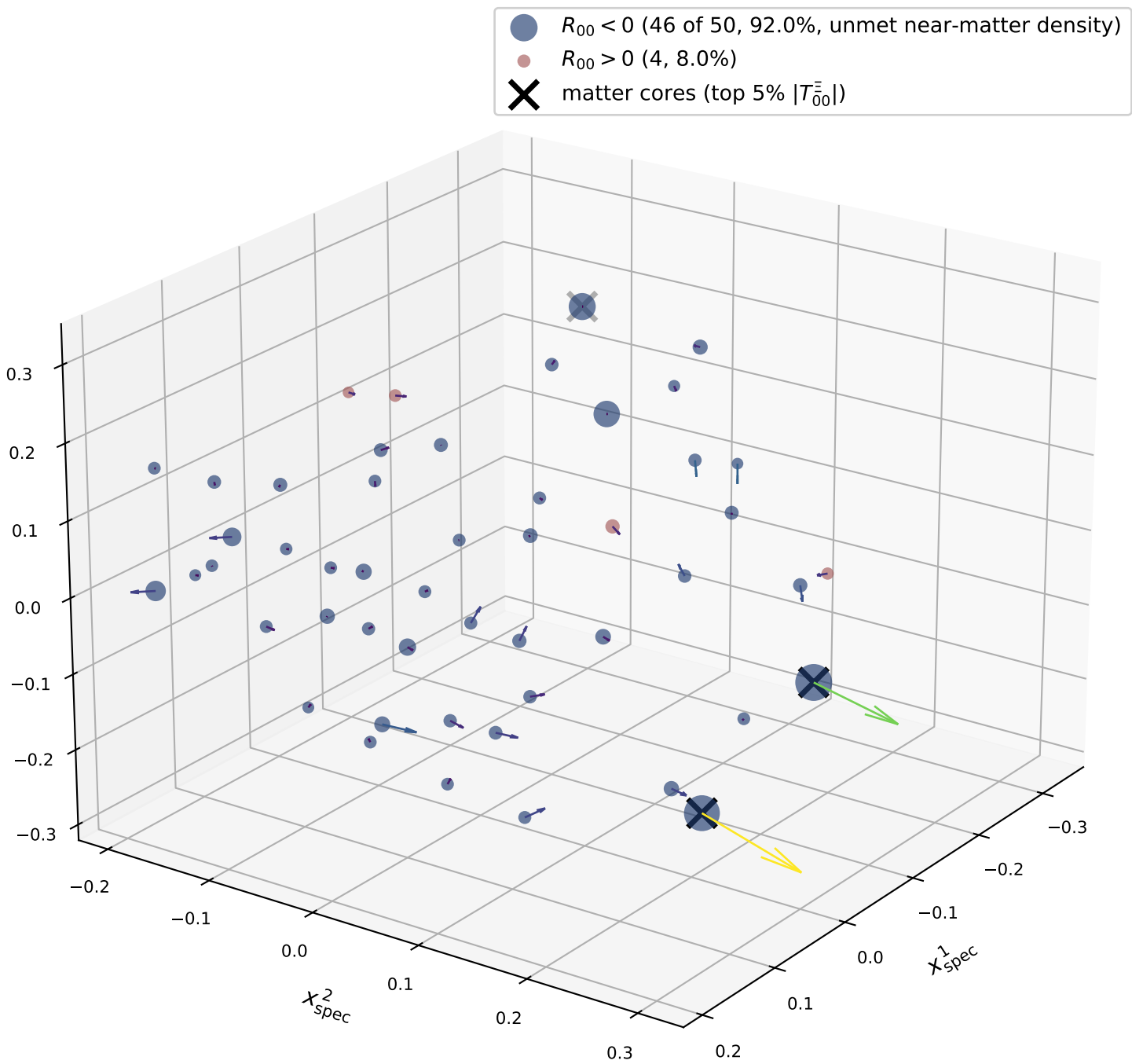
(a) P_5 , N=50
