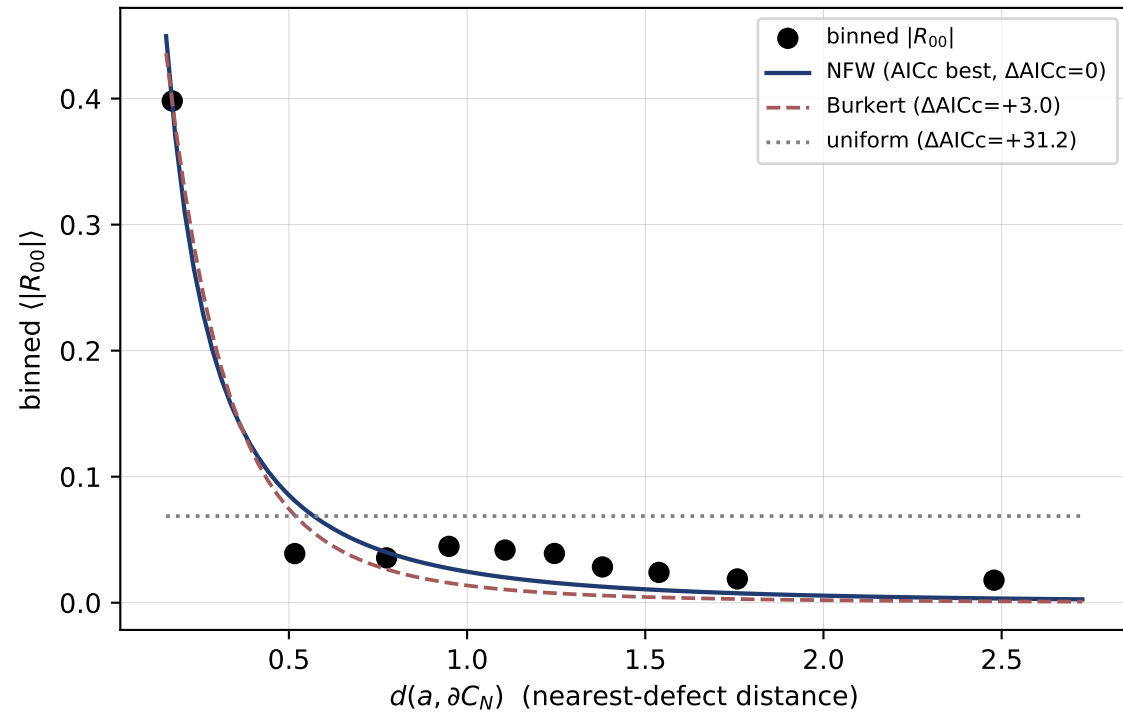
(a) Representative regime P5 ( N=50 ): NFW profile is AICc-preferred
