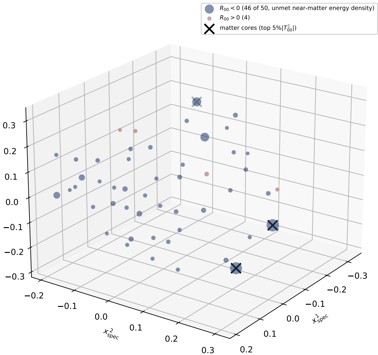
Energy-density residual R_{00}(a) in the spectral-frame spatial coordinates on a representative regime (P5, N=50 , single seed)
