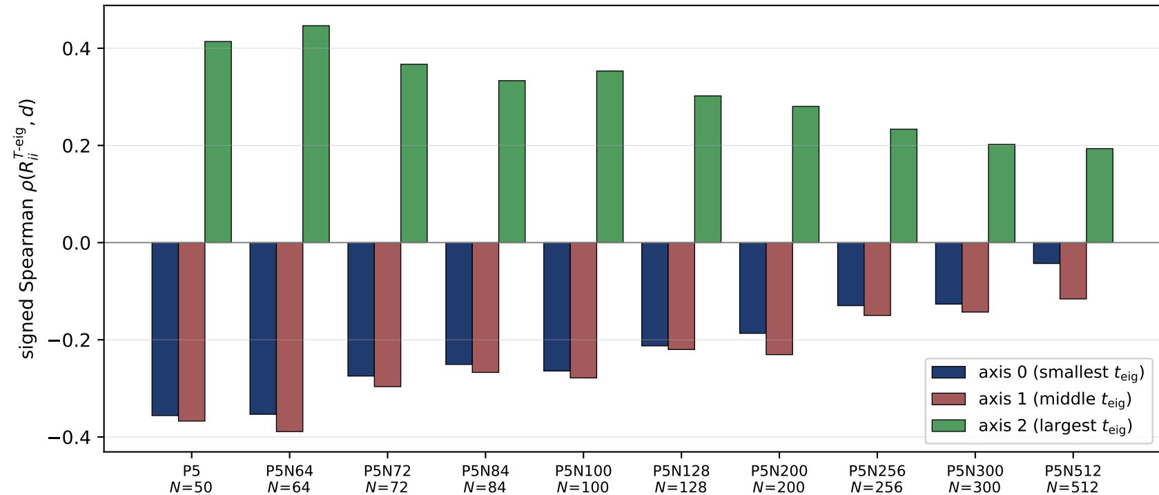
Genuine (2+1) sign pattern in the per-node T -eigenframe: axes 0,1 carry negative correlation, axis 2 carries positive correlation on 10/10 regimes
