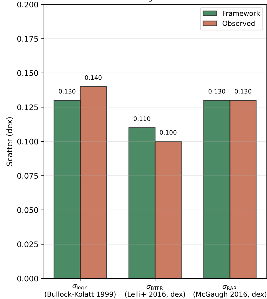
B2. Halo scaling-relation scatters
