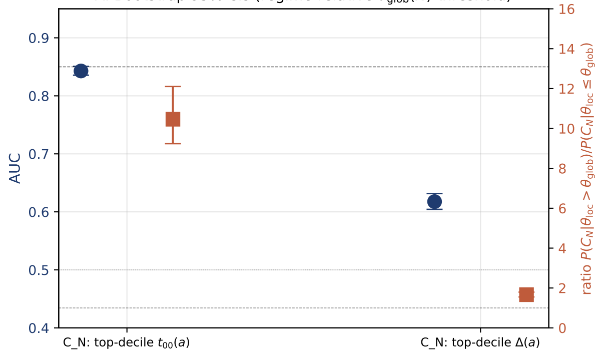
A. Bootstrap 95% CIs (regime-relative \theta_{\text{glob}}(N) threshold)
