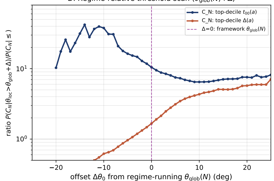
D. Regime-relative threshold scan ( \theta_{\text{glob}}(N) + \Delta )
