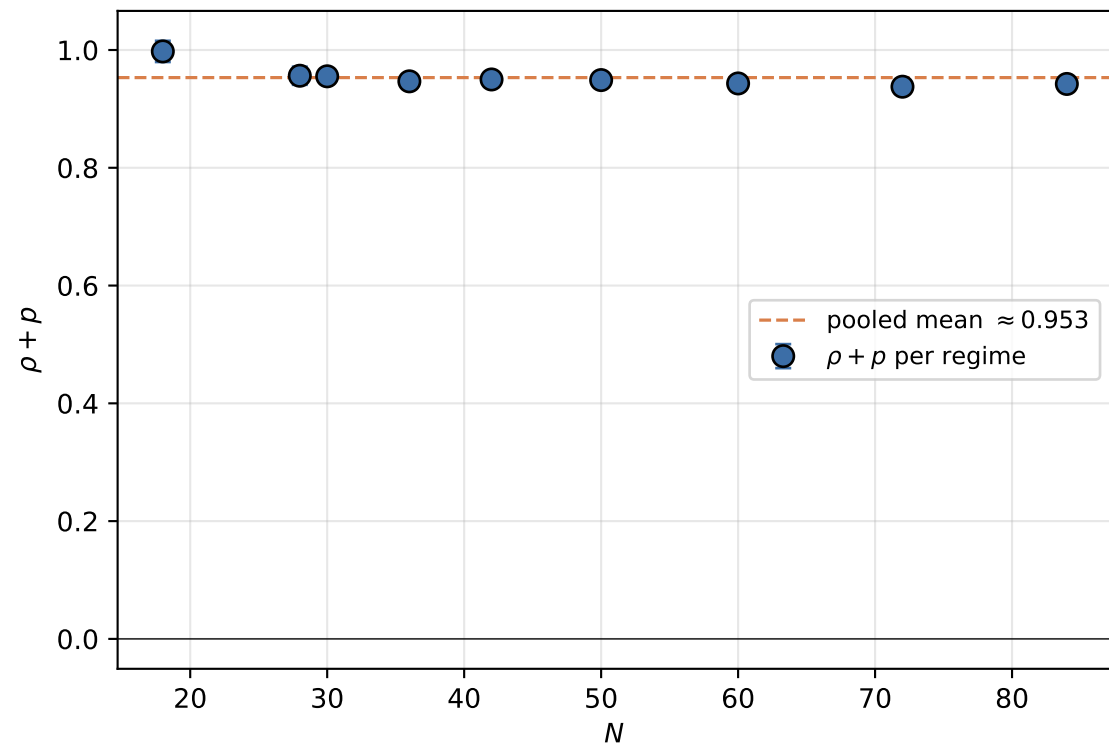
NEC margin: strongly satisfied (non-phantom solid, 1666\sigma above 0)
