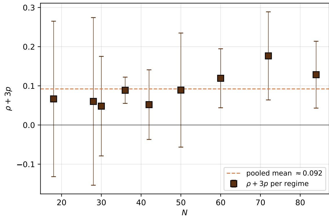
SEC margin: satisfied with 7.5\sigma above 0
