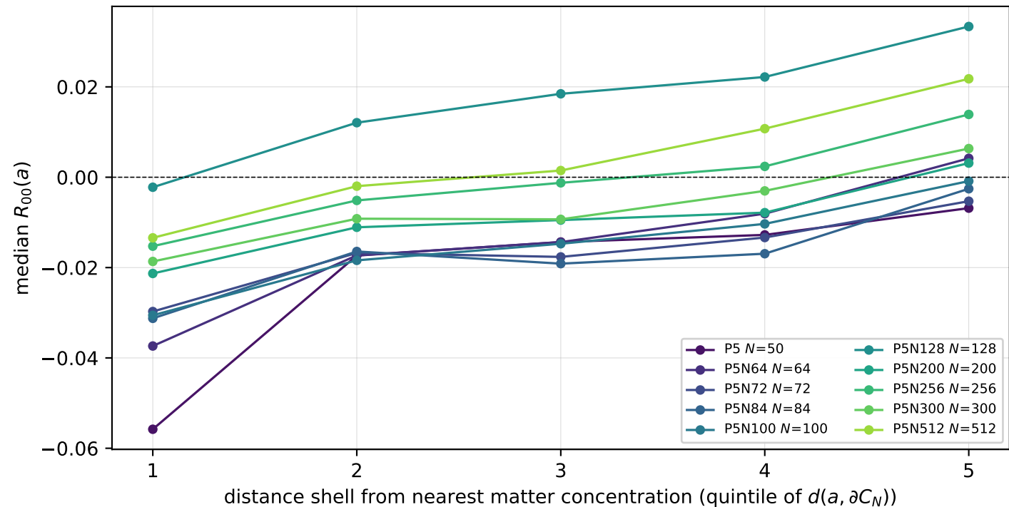
Residual energy density R_{00} approaches zero with increasing distance to the nearest matter concentration
